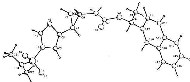
Figure 2. ORTEP drawing of 18 .
